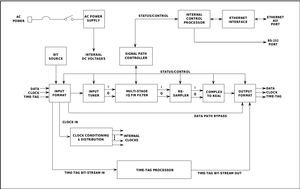
WJ-9488 Digital Sub-band Tuner Functional Block Diagram
